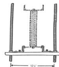
Edgewise Trapeze Product No. SBTE
