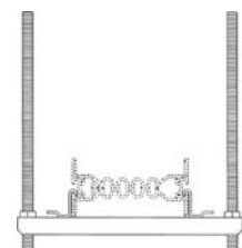
Trapeze Hanger for Edgewise Mounting
