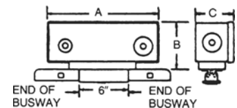
Center Feed Overslung
