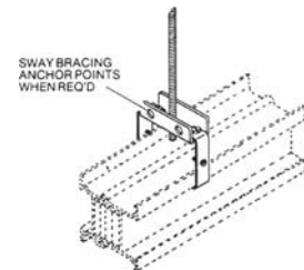
One-Stack Edgewise Product Number SBE45 (Up to 2000 Amp Max.)
