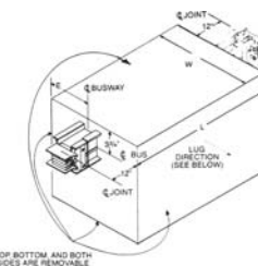
Center Tap Box: Feeder or Plug-in
