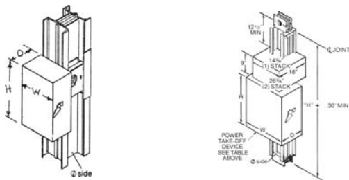
Fig. 1 Bolt on, Flex-A-Tap Fig. 2 Flatwise PTO Section
