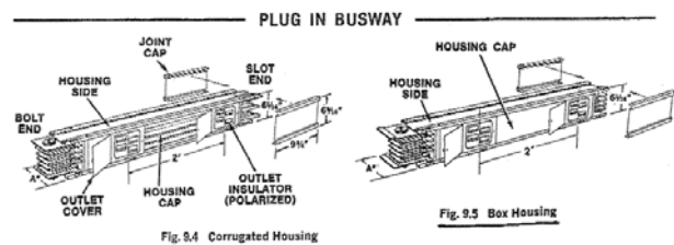
Fig. 9.4 Corrugated Housing
